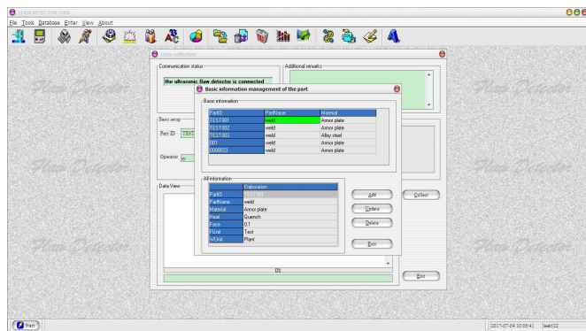
Data Management
