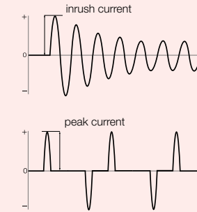
Measure the inrush current when copiers and similar equipment are started
